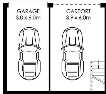
LOWER LEVEL
